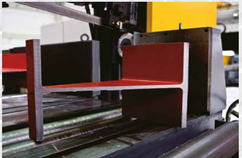
ROTATING SAW
